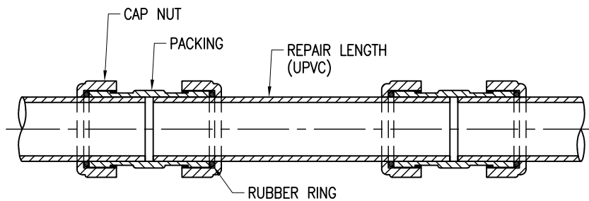
SIMPLE JOINT
