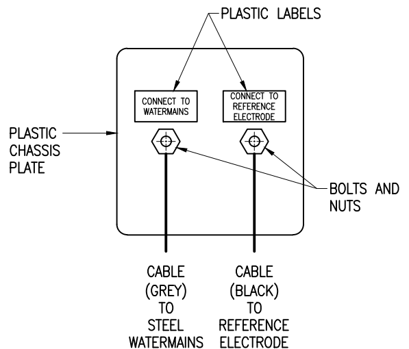
DETAILS OF TYPICAL TEST STATION INTERIOR
