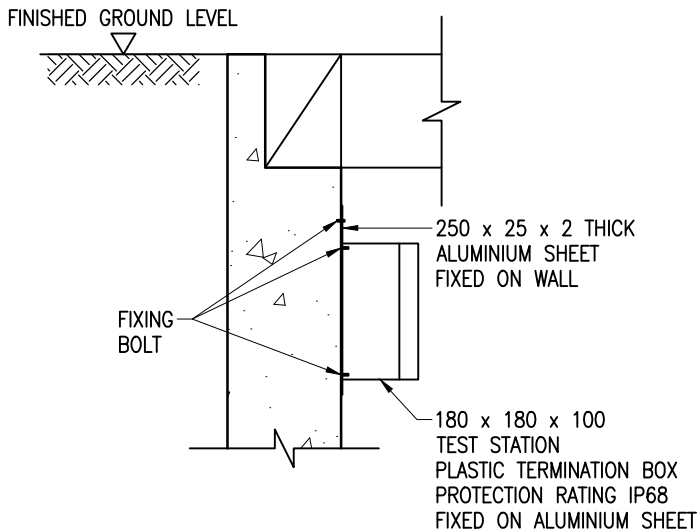
DETAILS OF TEST STATION FIXING
