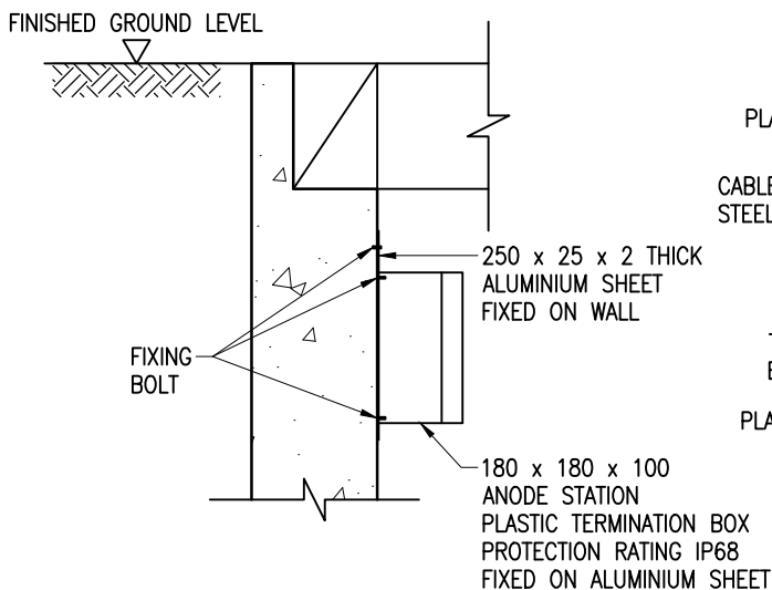
DETAILS OF ANODE STATION FIXING
