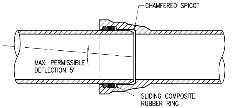
TYTON JOINT
