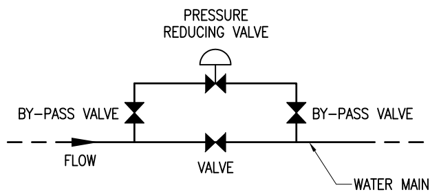
CONFIGURATION OF PRESSURE REDUCING VALVE
