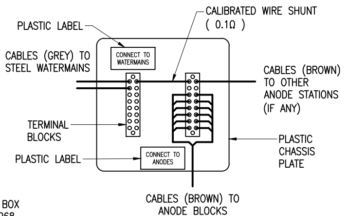
DETAILS OF TYPICAL ANODE STATION INTERIOR
