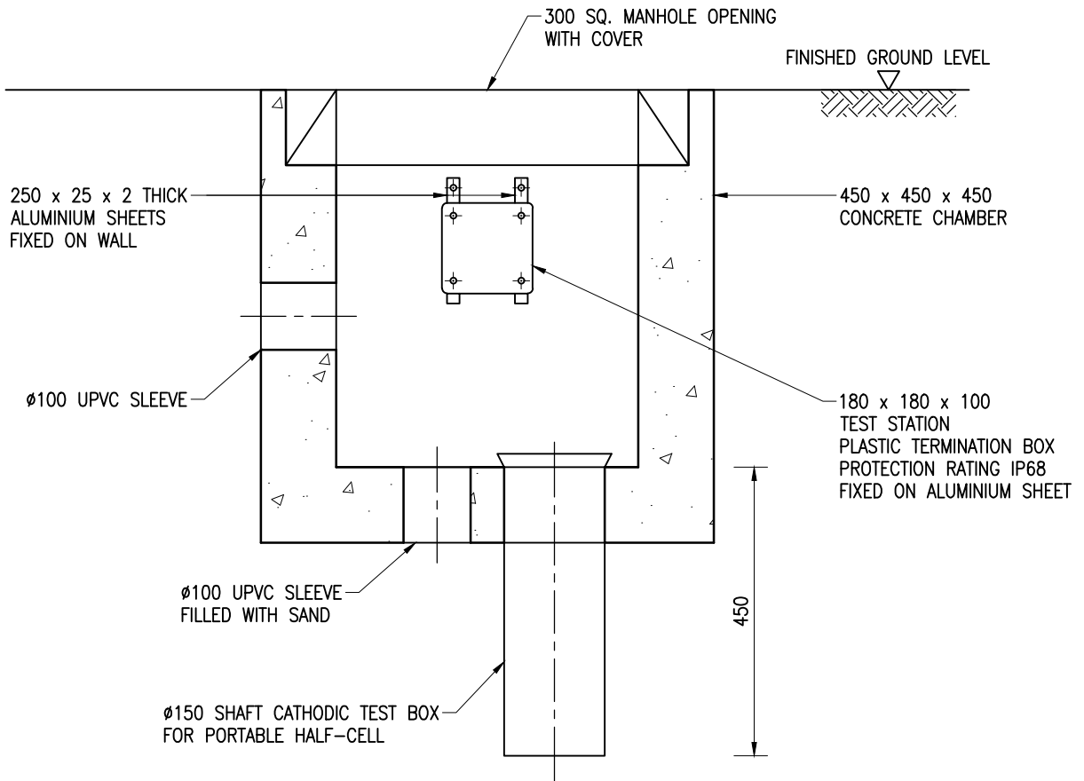
DETAILS OF TEST STATION
