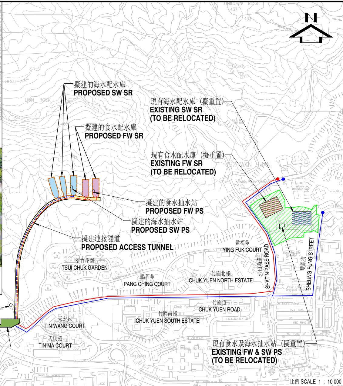
擬建於連接隧道入口的通風設施及其他相關機電設施 PROPOSED VENTILATION AND OTHER ASSOCIATED E&M FACILITIES AT ACCESS TUNNEL PORTAL AREA
