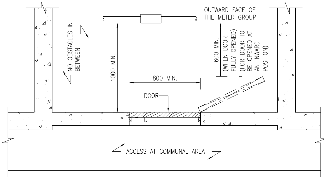
SECTIONAL PLAN
